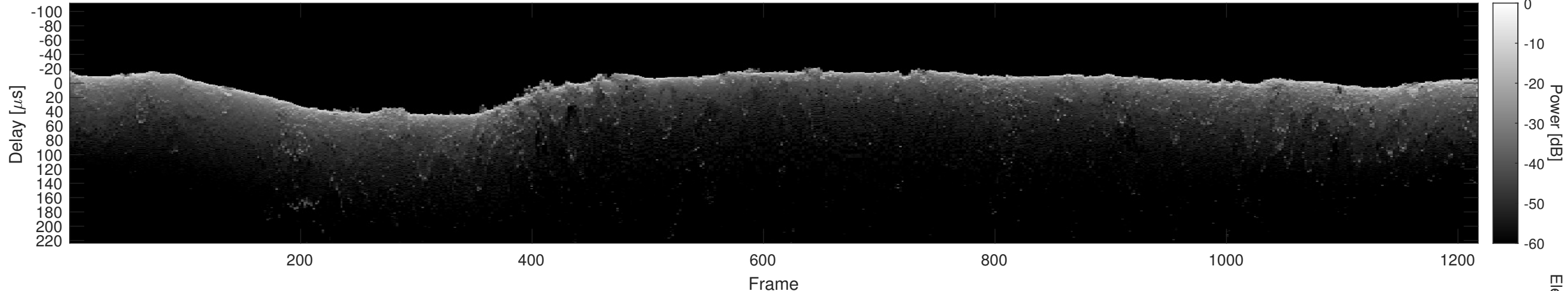
Orbit 22963, Cluttergram
