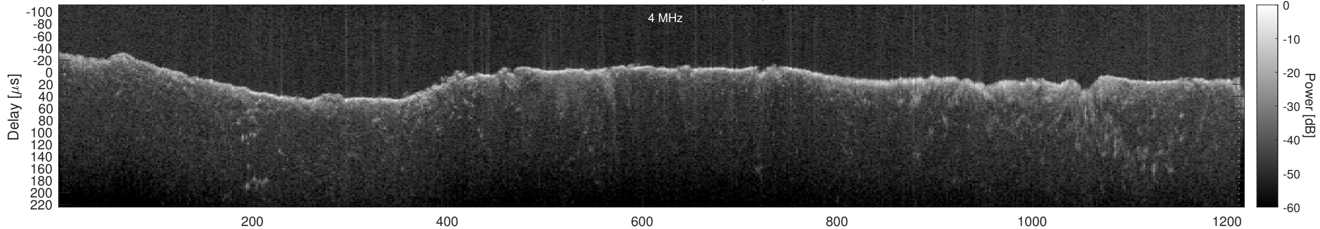
Orbit 22963, Window, Channel 2, Optimized
