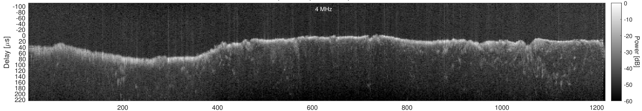
Orbit 22963, Window, Channel 2, Chapman
