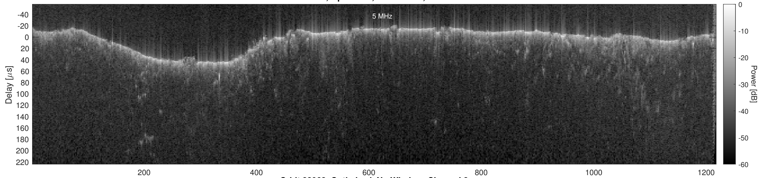
Orbit 22963, Optimized, No Window, Channel 2
