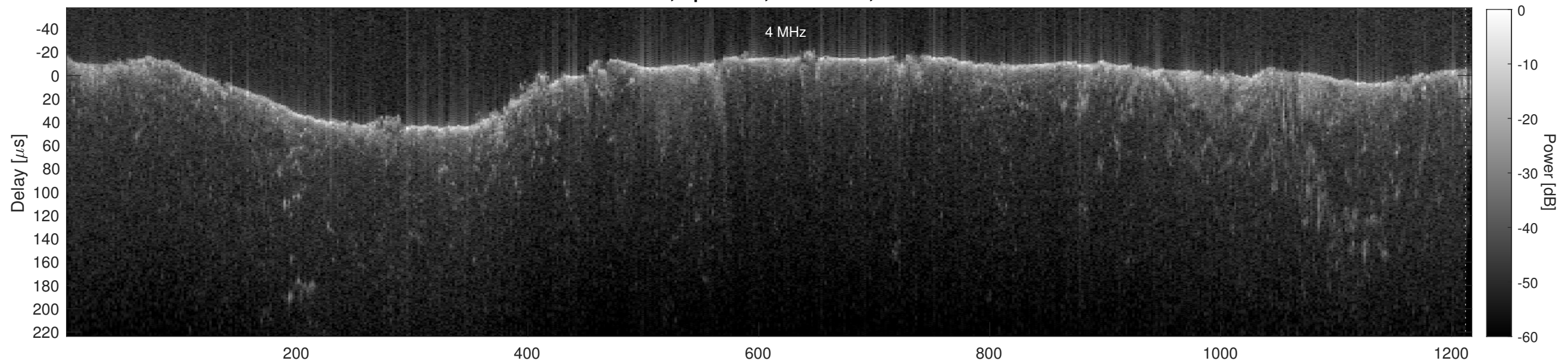
Orbit 22963, Cluttergram
