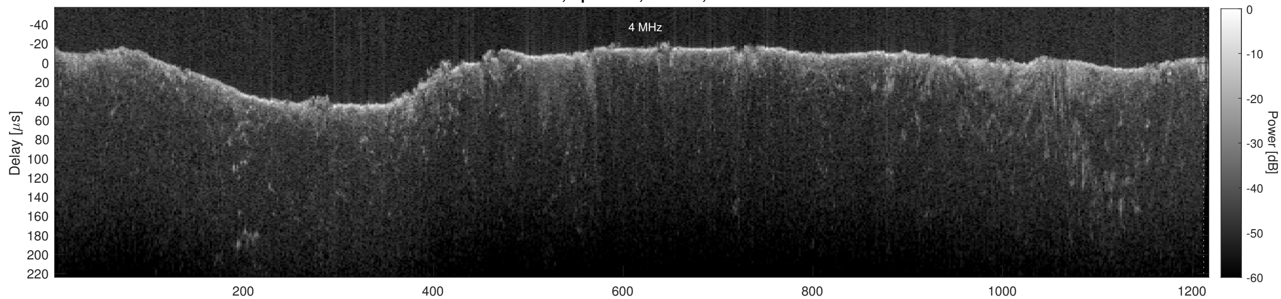
Orbit 22963, Cluttergram
