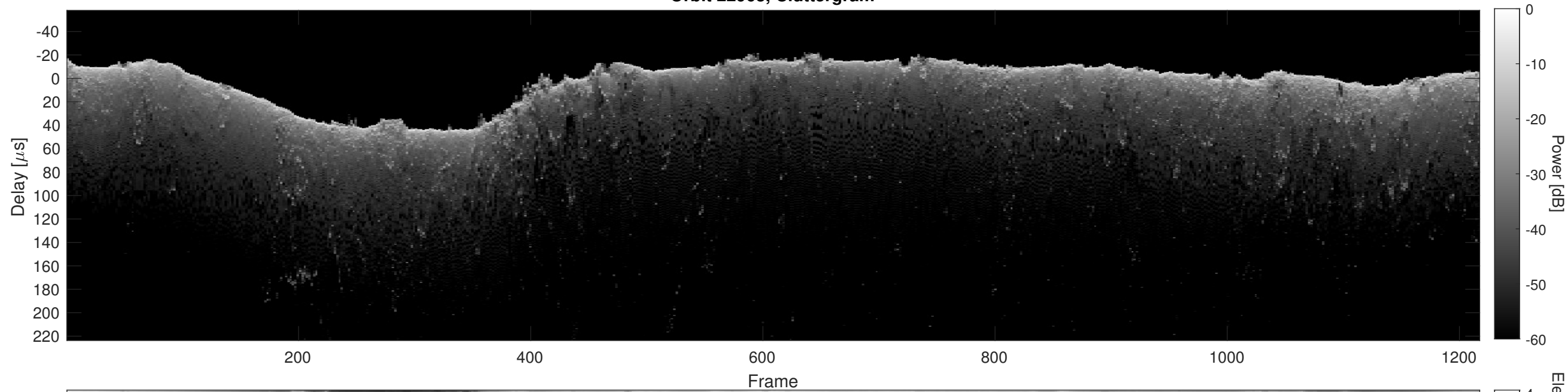
Orbit 22963, Cluttergram
