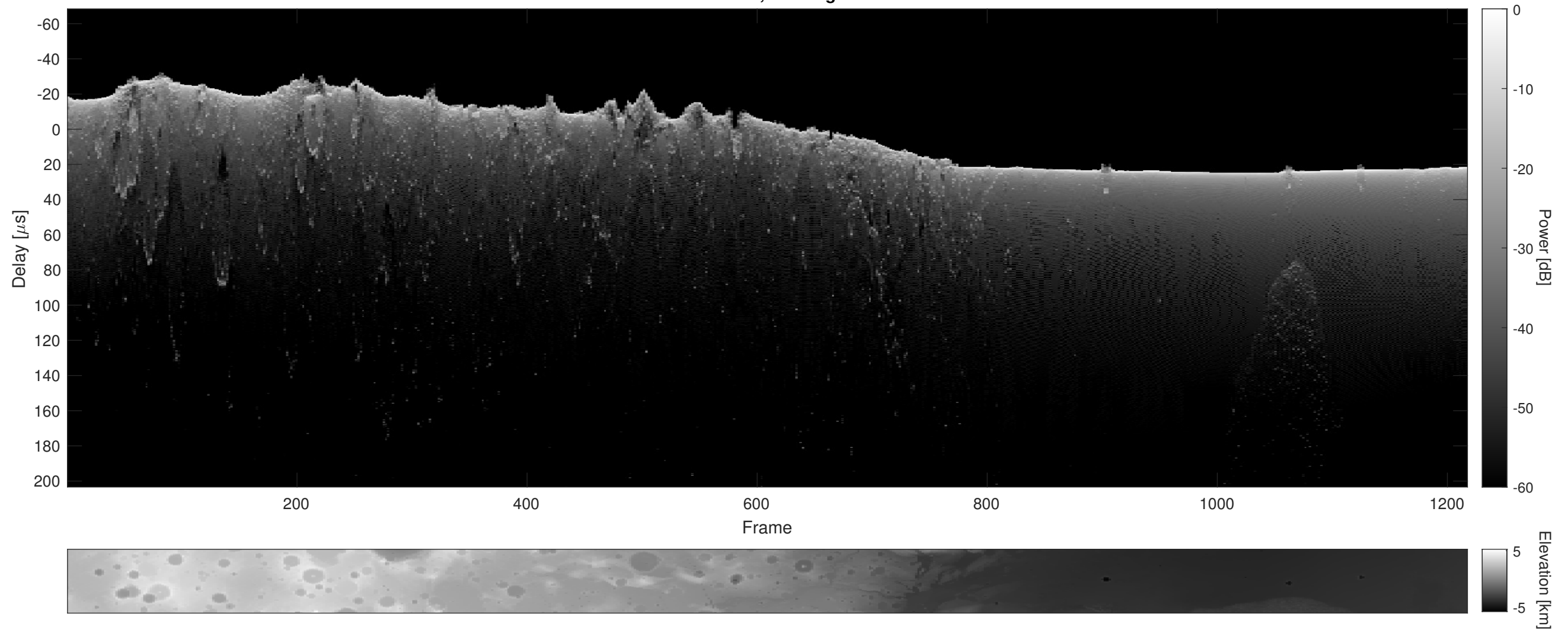
Orbit 22965, Cluttergram
