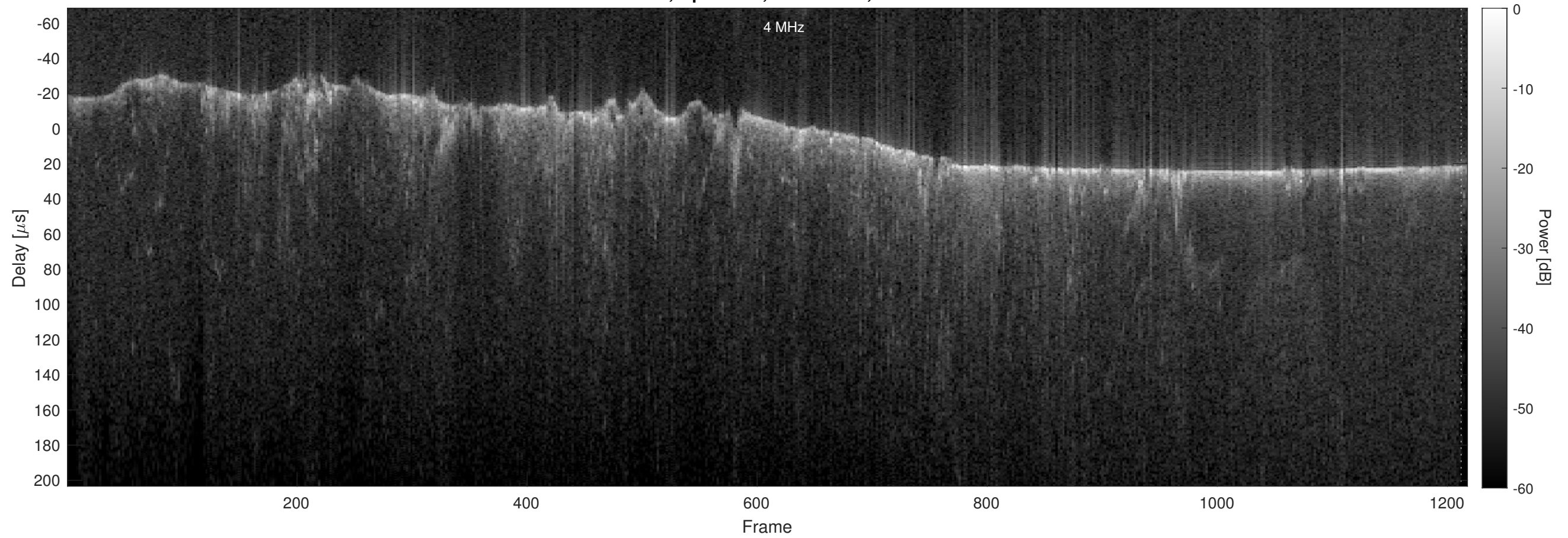
Orbit 22965, Optimized, No Window, Channel 2
