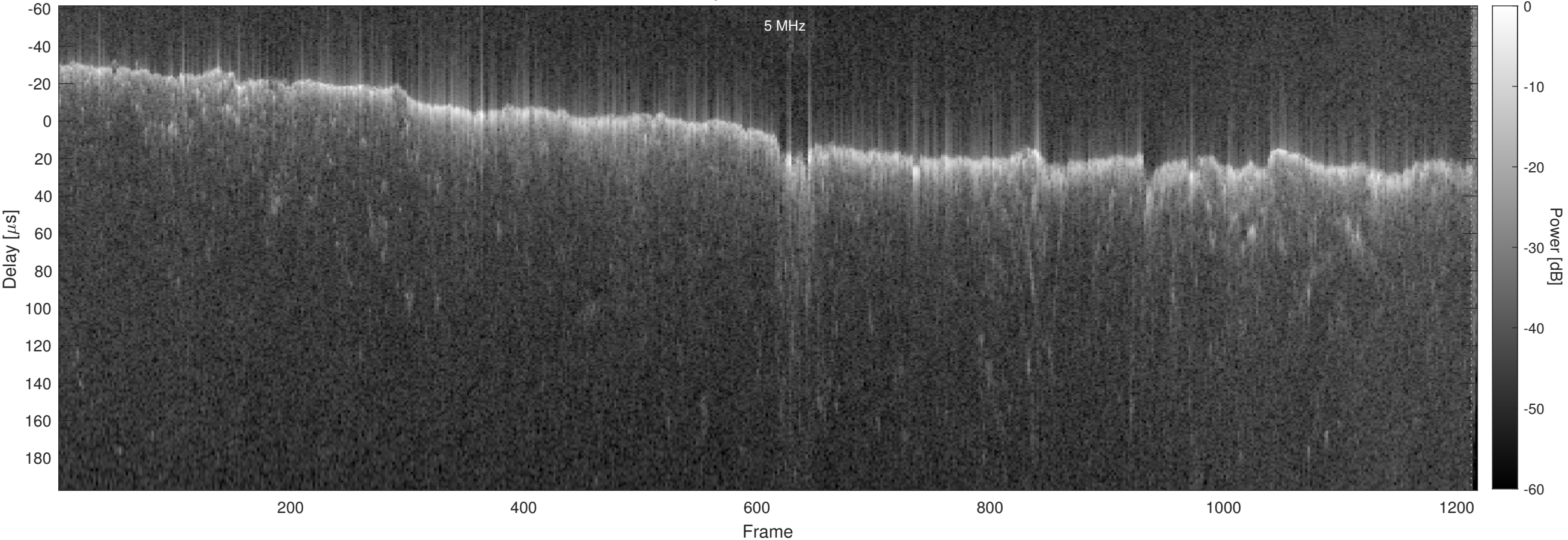
Orbit 22967, Chapman, No Window, Channel 2
