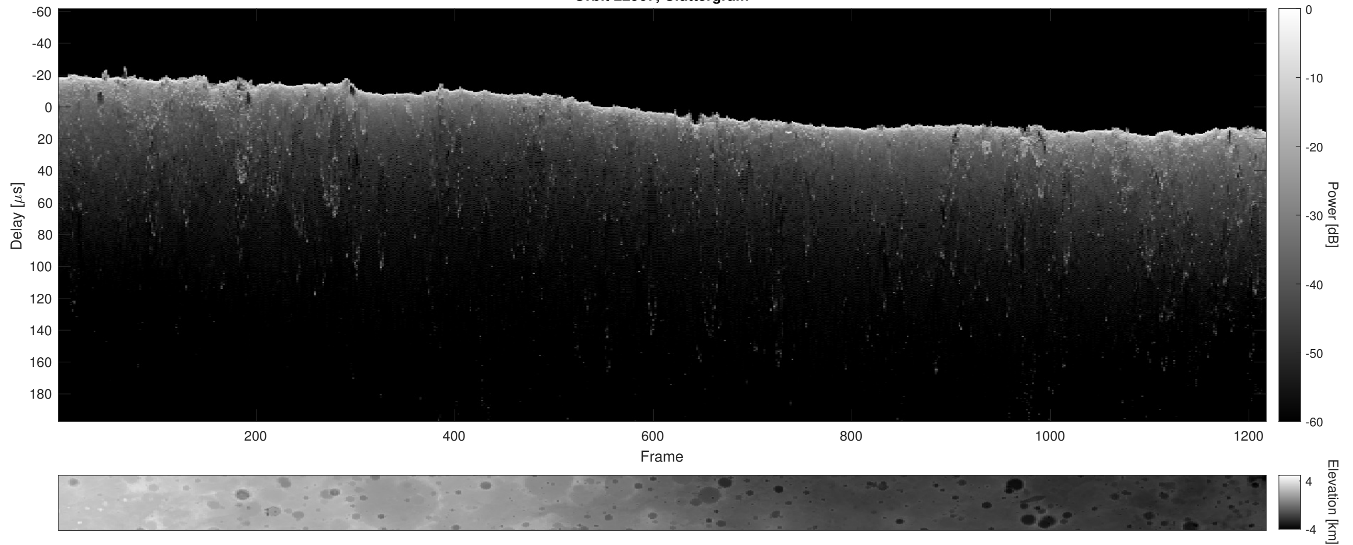
Orbit 22967, Cluttergram
