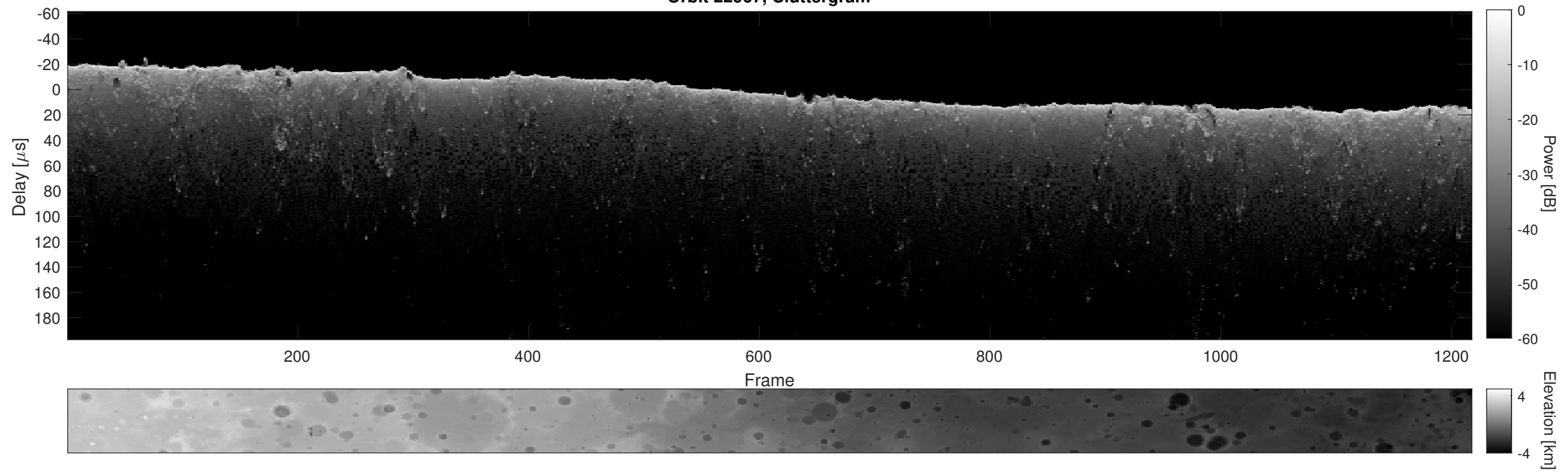
Orbit 22967, Cluttergram
