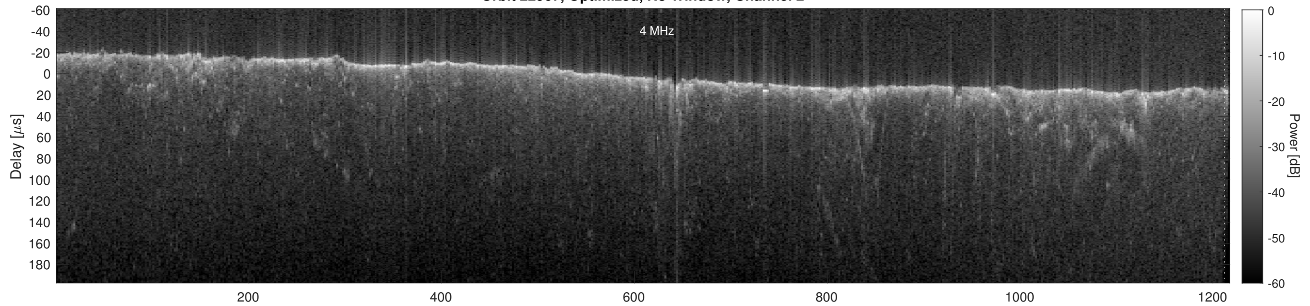
Orbit 22967, Cluttergram
