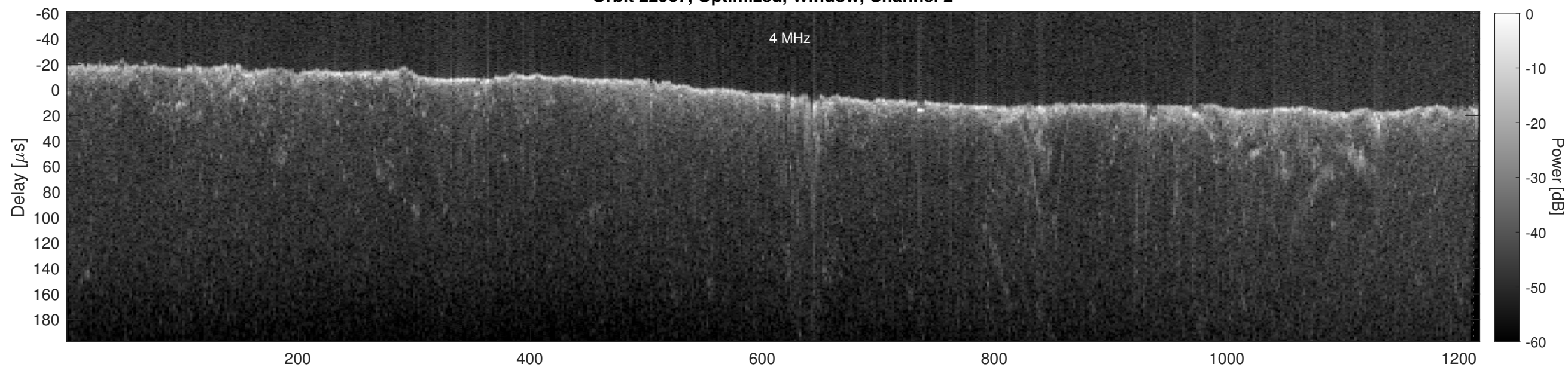
Orbit 22967, Cluttergram
