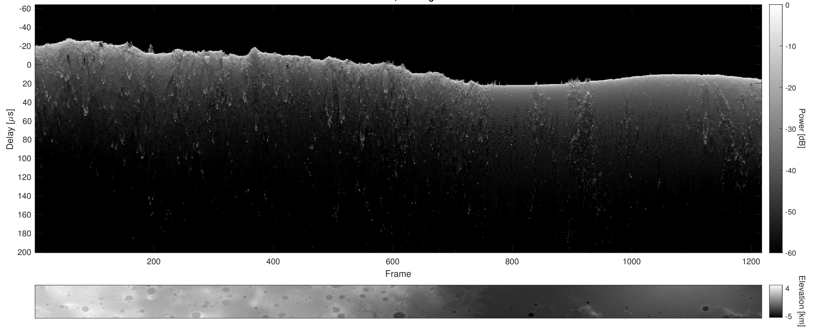
Orbit 22969, Cluttergram
