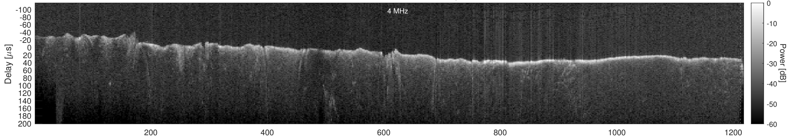
Orbit 22969, Window, Channel 2, Optimized
