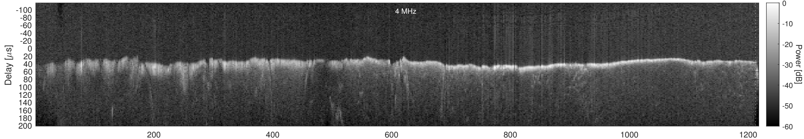
Orbit 22969, Window, Channel 2, Chapman
