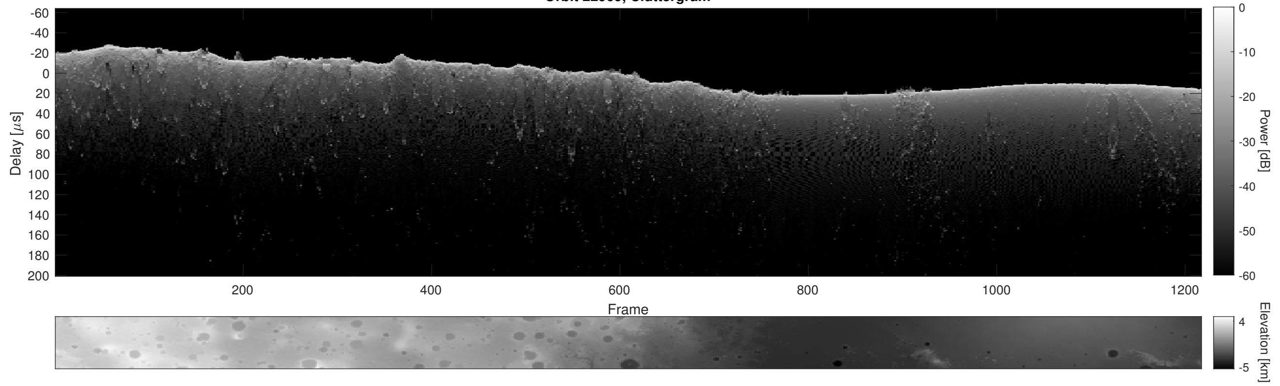
Orbit 22969, Cluttergram
