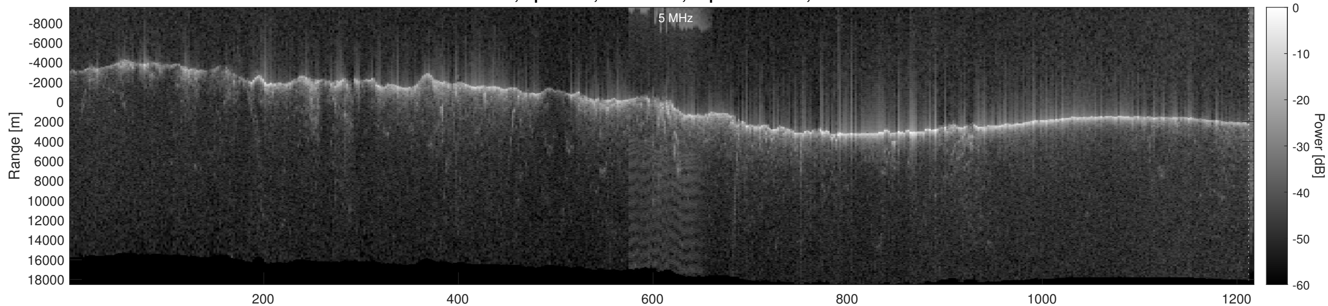
Orbit 22969, Optimized, No Window, Depth-Corrected, Channel 2
