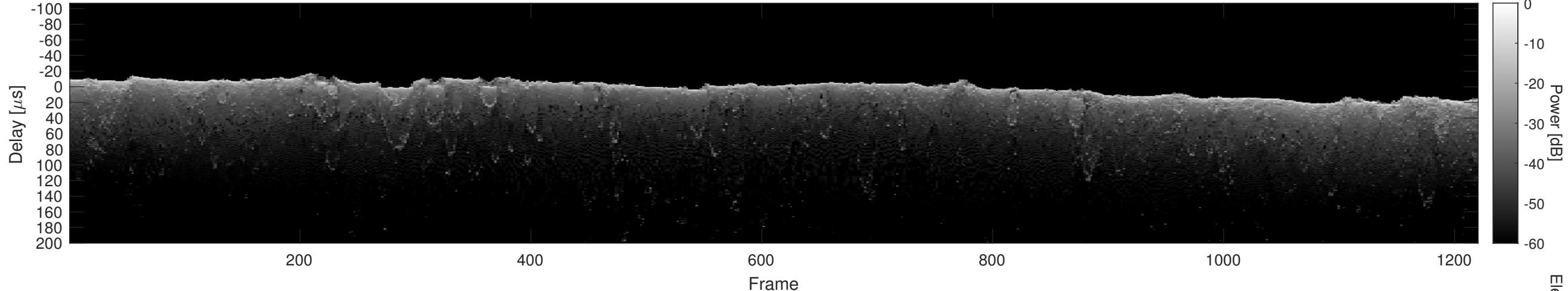
Orbit 23002, Cluttergram
