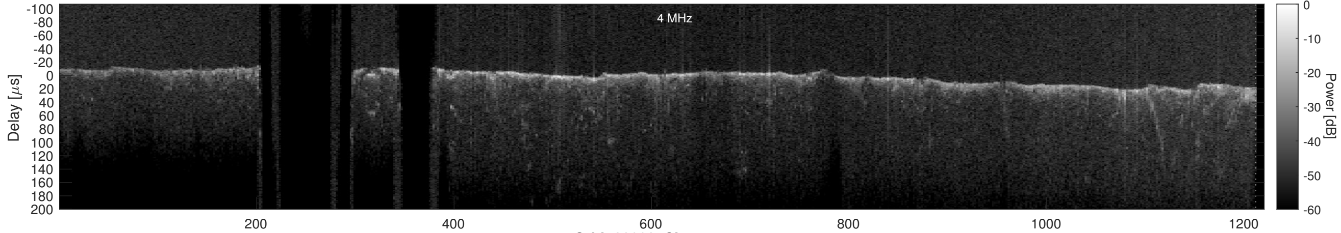
Orbit 23002, Cluttergram
