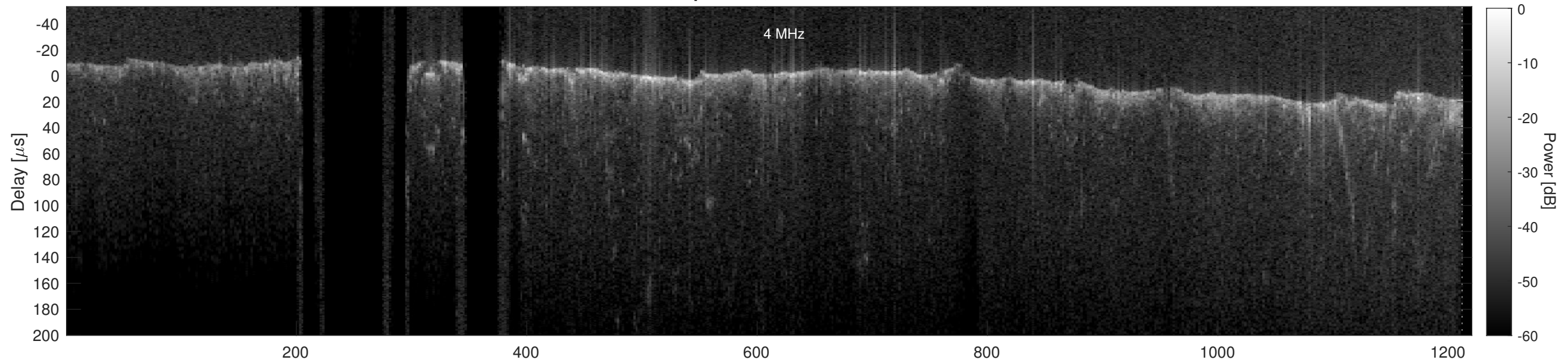
Orbit 23002, Cluttergram
