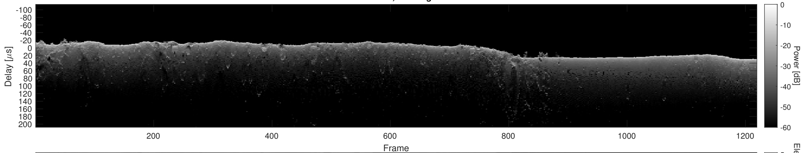
Orbit 23008, Cluttergram
