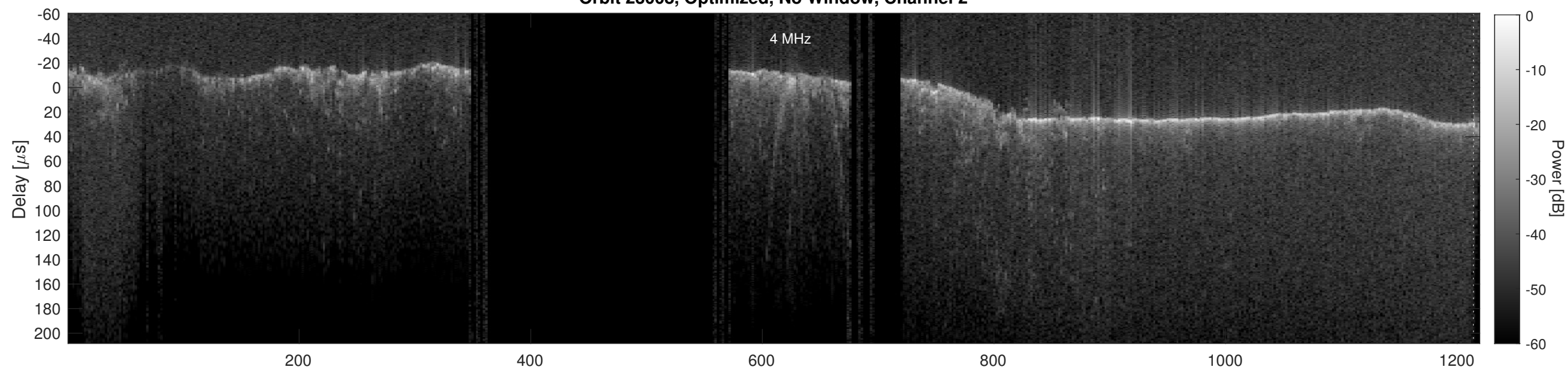
Orbit 23008, Cluttergram
