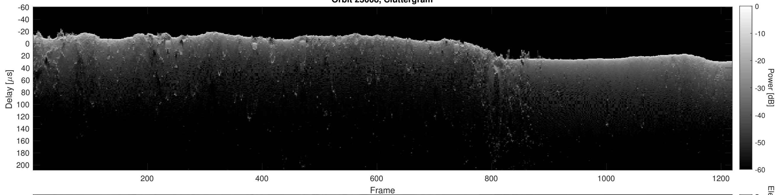
Orbit 23008, Cluttergram
