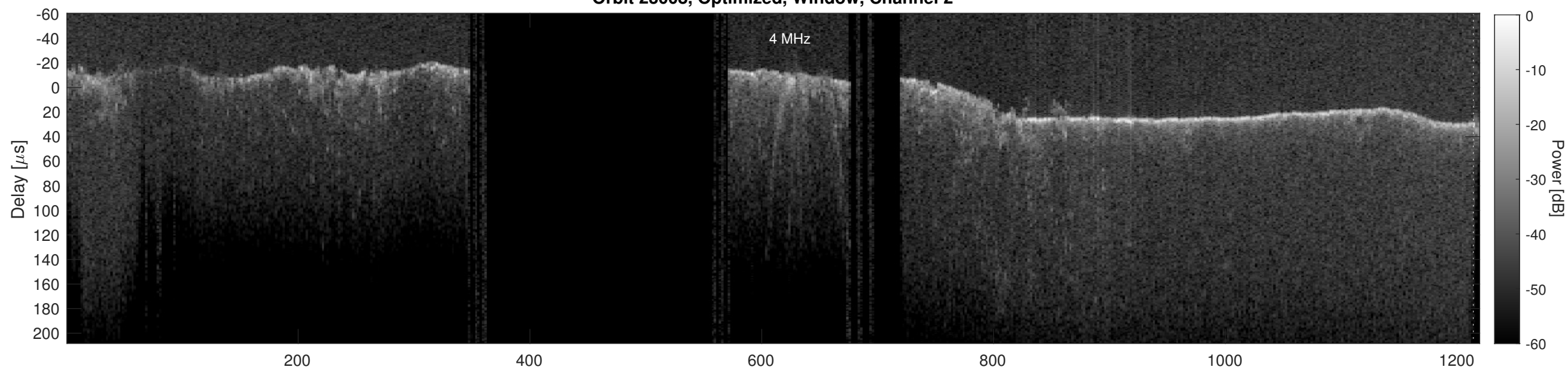
Orbit 23008, Cluttergram
