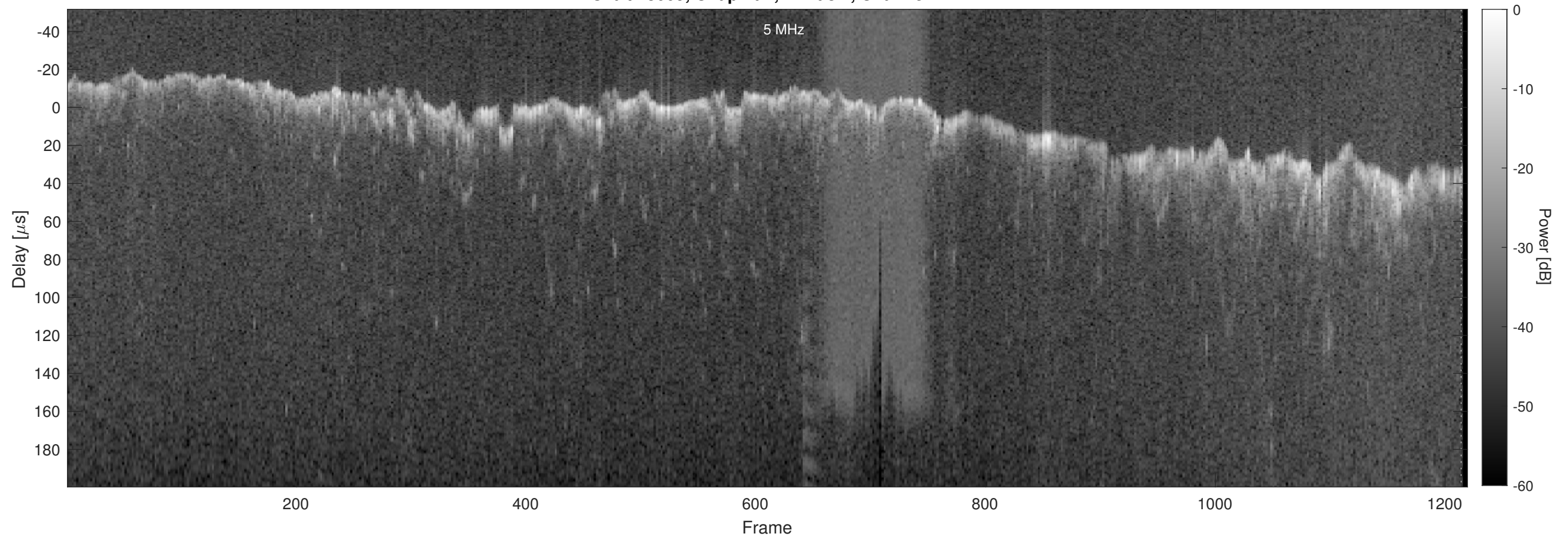
Orbit 23009, Chapman, Window, Channel 2
