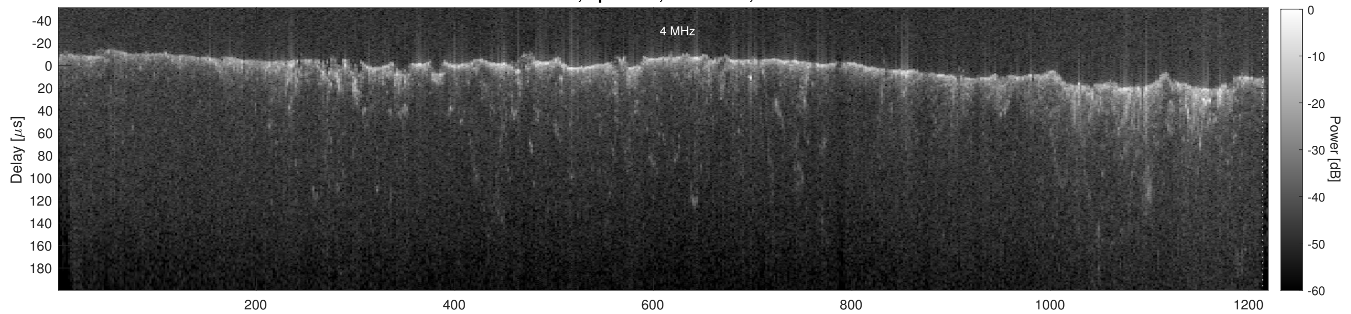
Orbit 23009, Cluttergram
