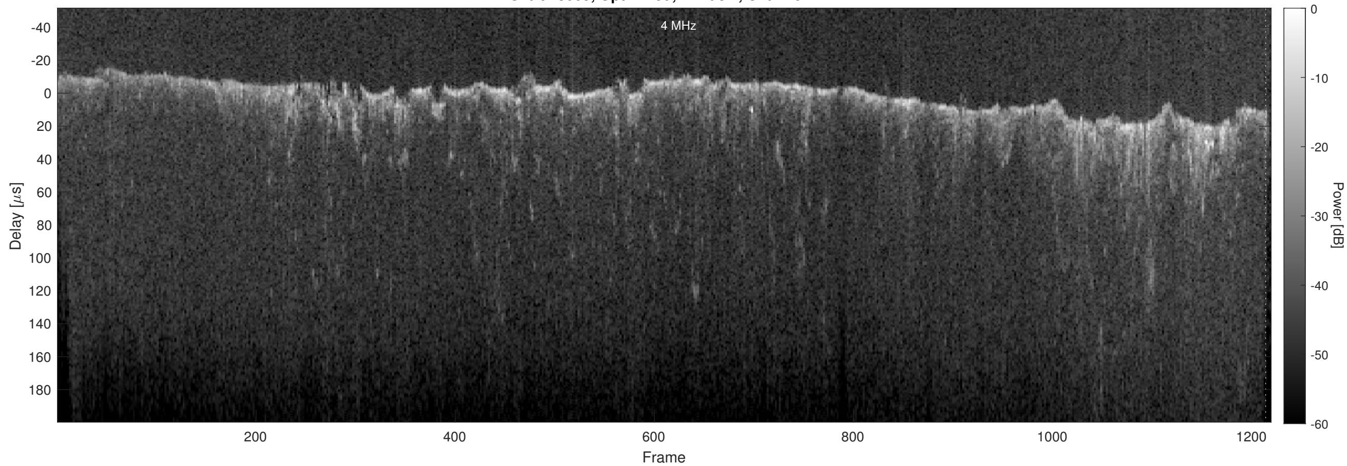
Orbit 23009, Optimized, Window, Channel 2
