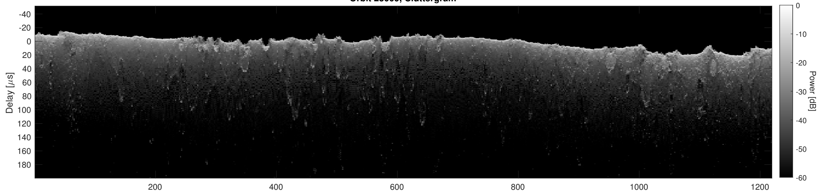
Orbit 23009, Cluttergram
