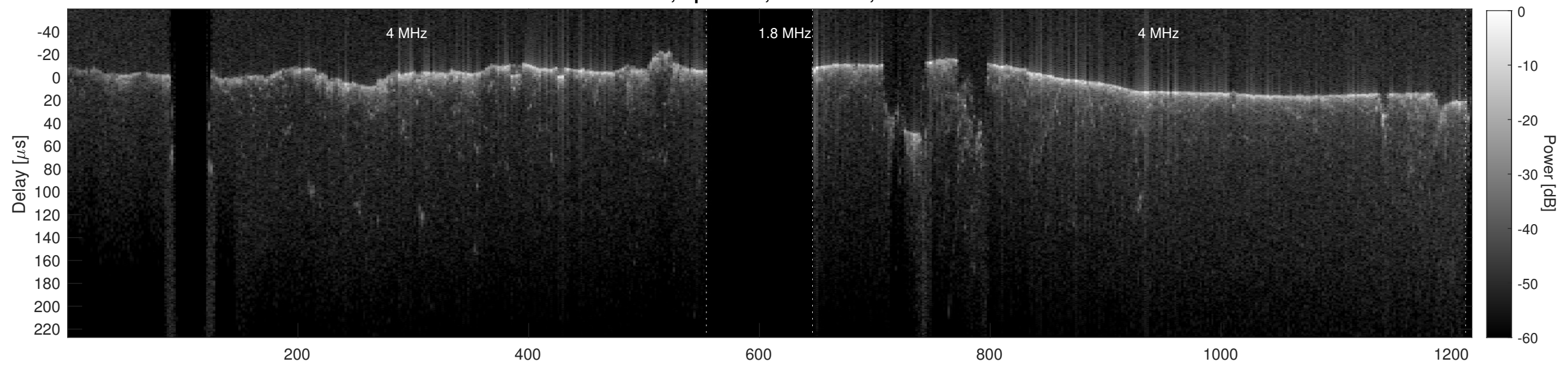
Orbit 23010, Cluttergram
