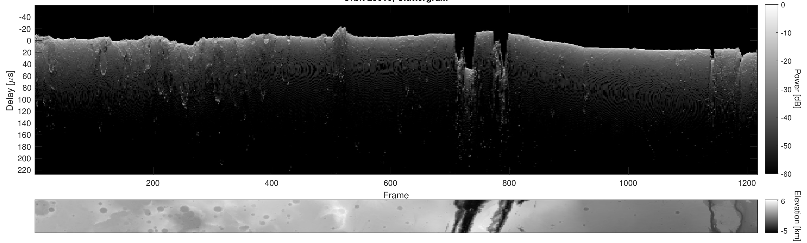
Orbit 23010, Cluttergram
