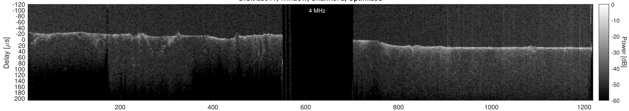
Orbit 23011, Cluttergram
