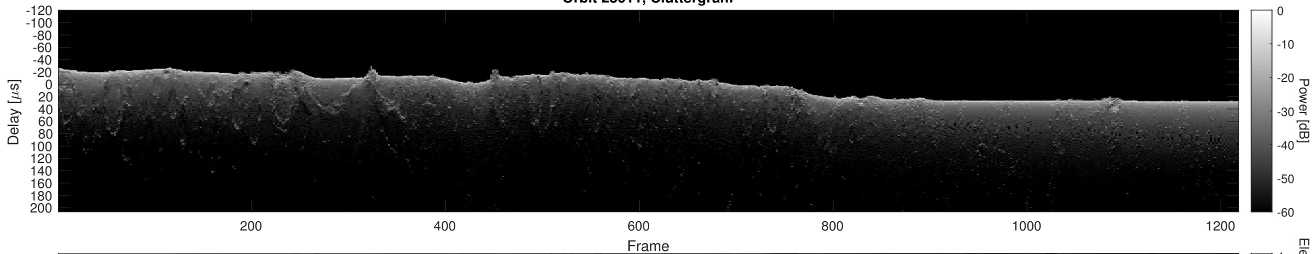
Orbit 23011, Cluttergram
