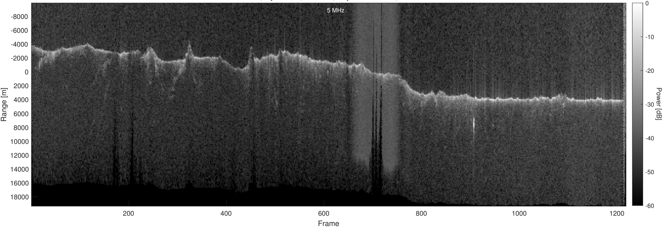
Orbit 23011, Optimized, Window, Depth-Corrected, Channel 2
