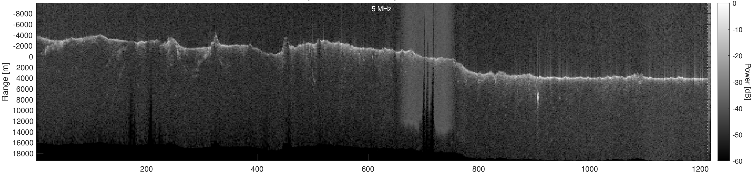
Orbit 23011, Optimized, Window, Depth-Corrected, Channel 2
