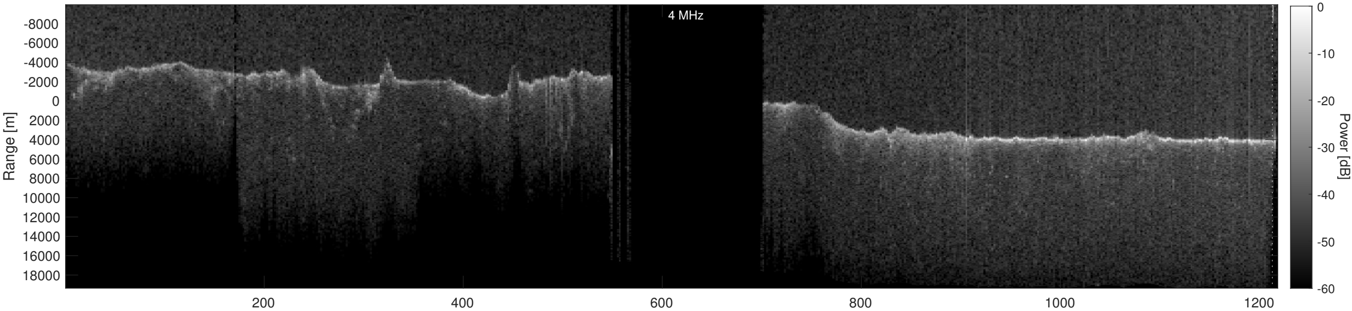
Orbit 23011, Depth-Corrected Cluttergram
