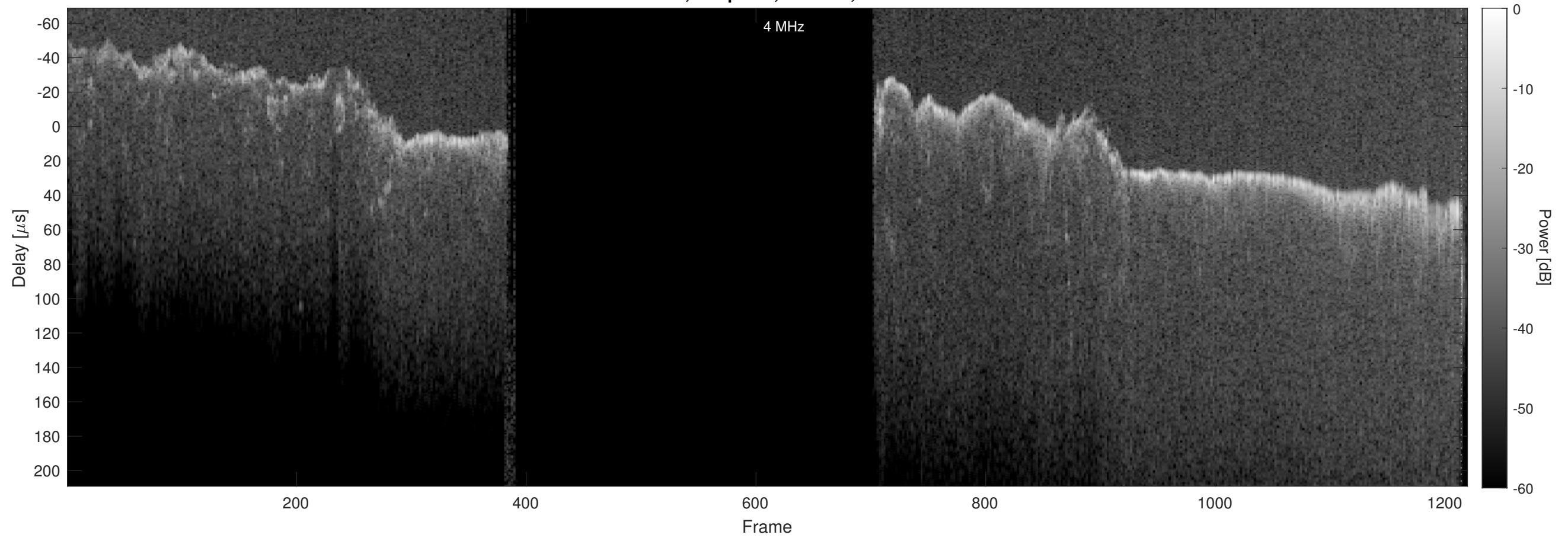
Orbit 23012, Chapman, Window, Channel 2
