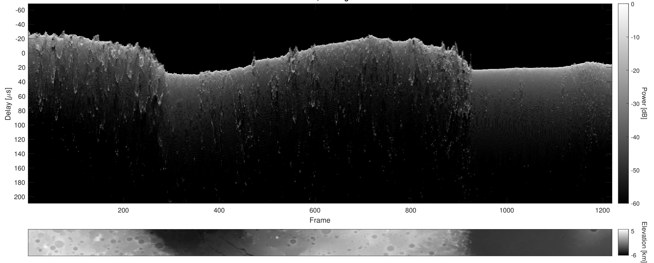
Orbit 23012, Cluttergram
