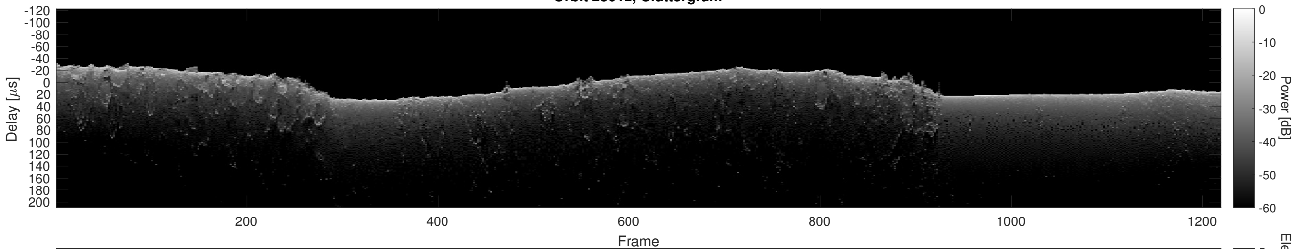
Orbit 23012, Cluttergram
