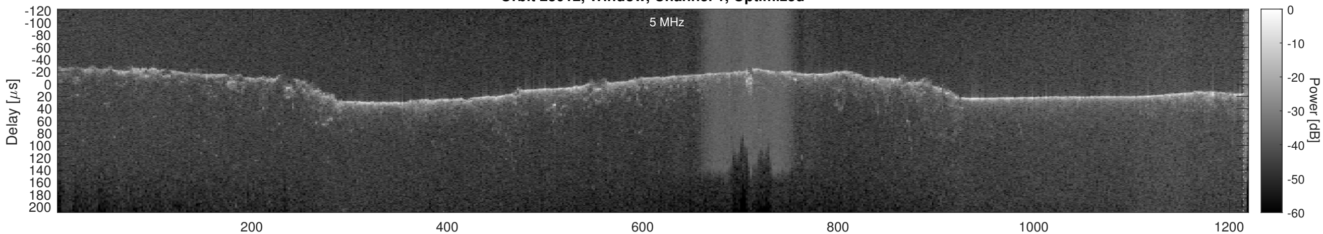
Orbit 23012, Cluttergram
