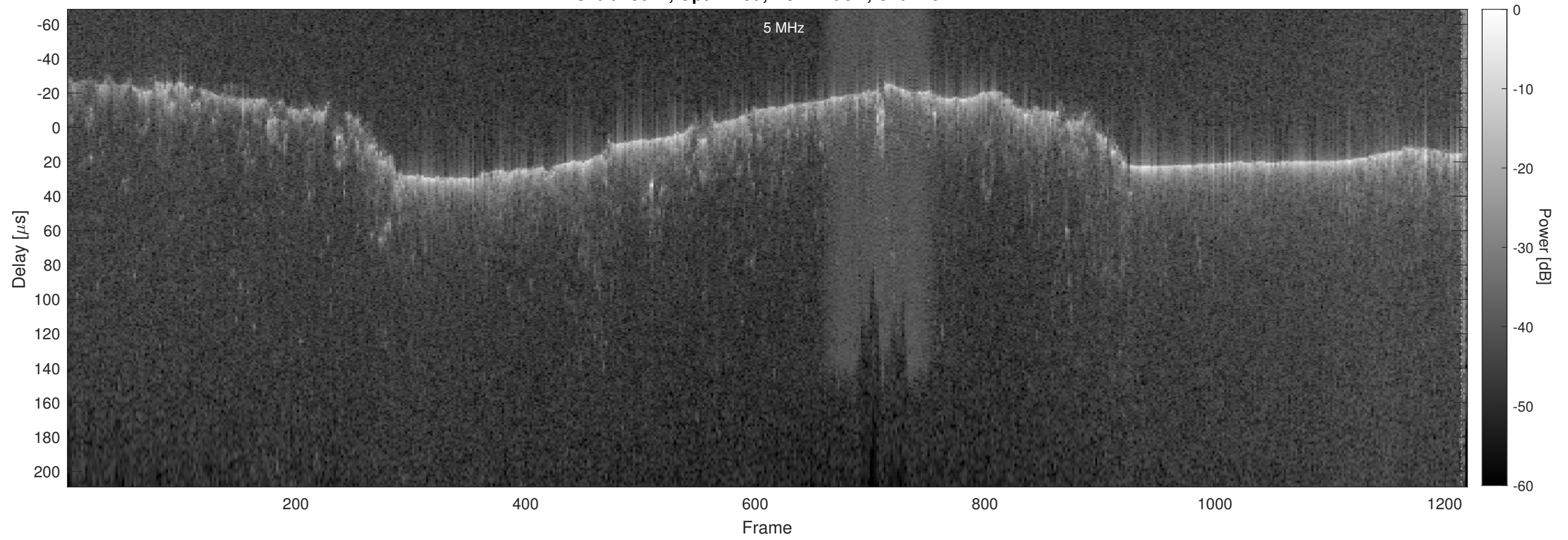
Orbit 23012, Optimized, No Window, Channel 2
