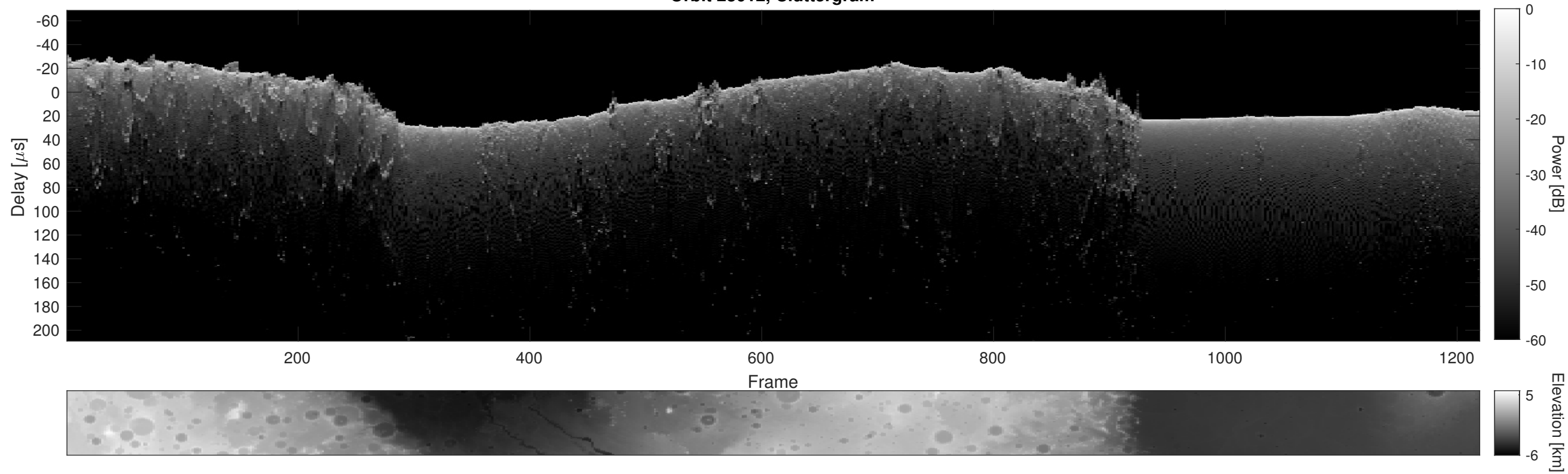
Orbit 23012, Cluttergram
