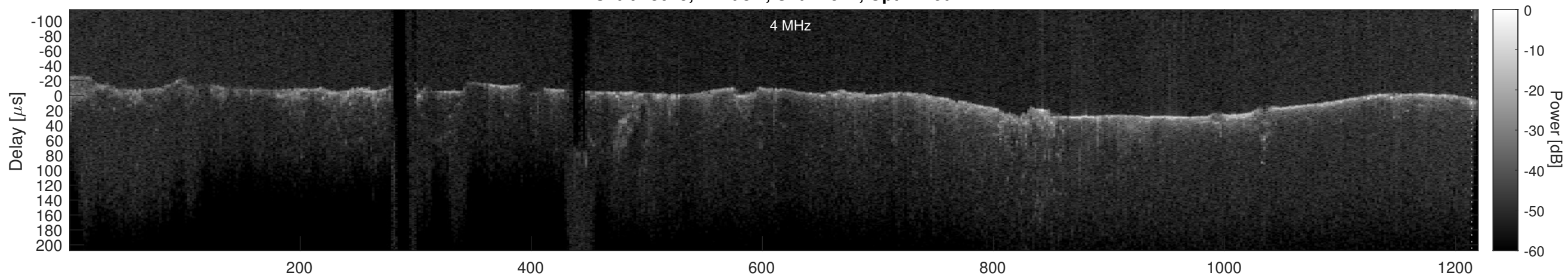
Orbit 23015, Cluttergram
