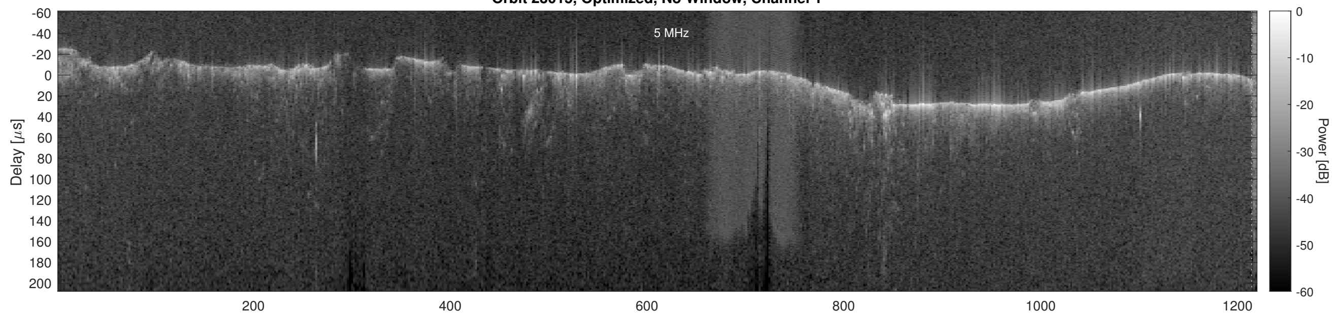
Orbit 23015, Optimized, No Window, Channel 2
