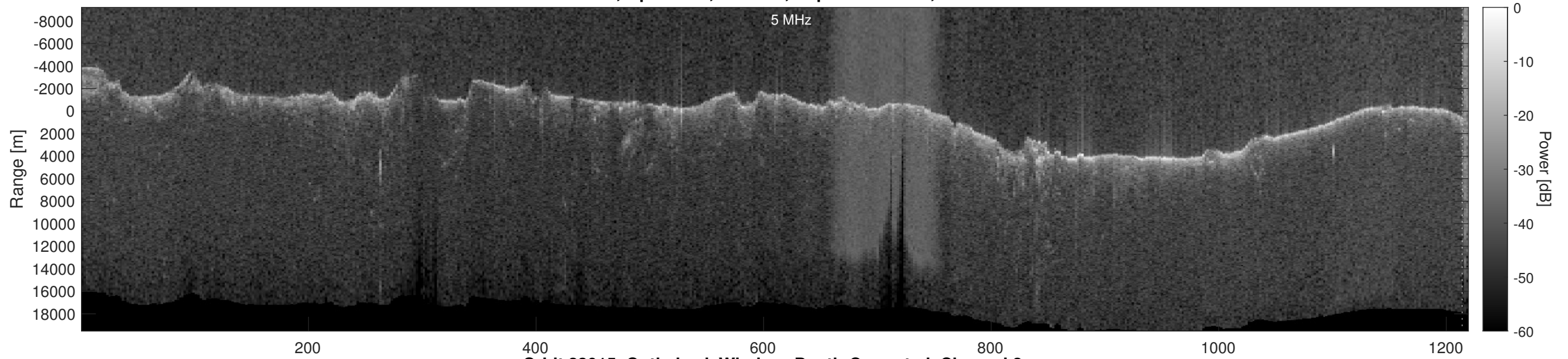
Orbit 23015, Optimized, Window, Depth-Corrected, Channel 2
