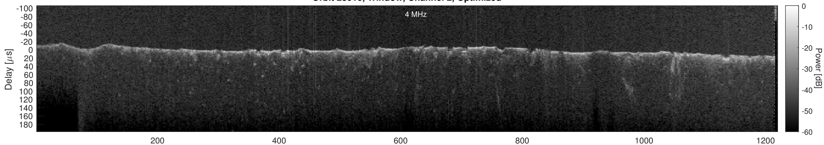
Orbit 23016, Cluttergram
