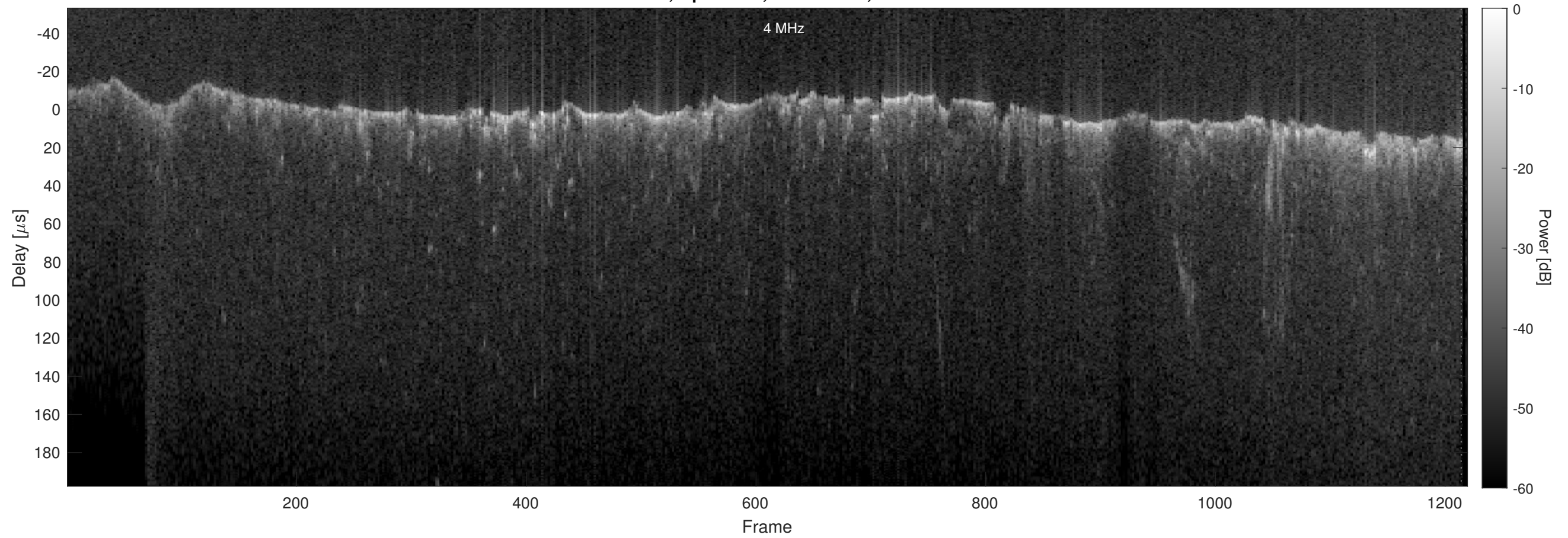
Orbit 23016, Optimized, No Window, Channel 2
