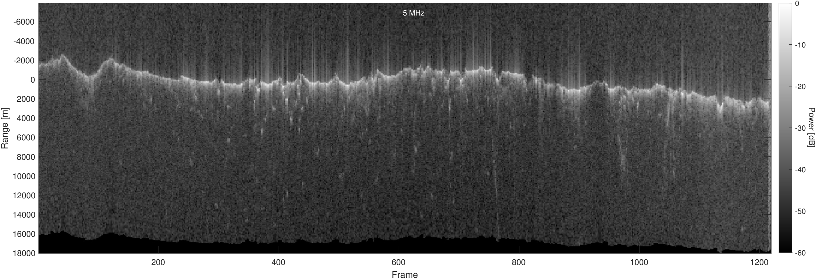
Orbit 23016, Optimized, No Window, Depth-Corrected, Channel 2
