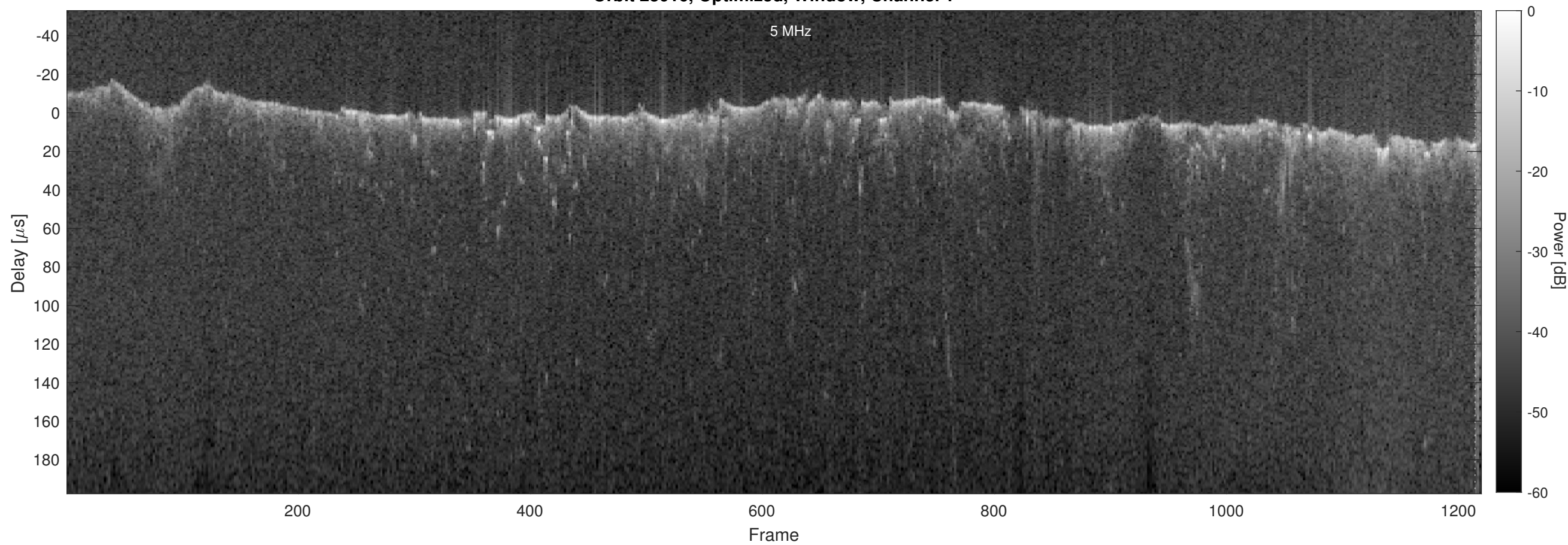
Orbit 23016, Optimized, Window, Channel 2
