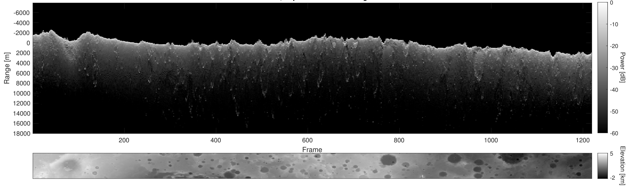
Orbit 23016, Depth-Corrected Cluttergram
