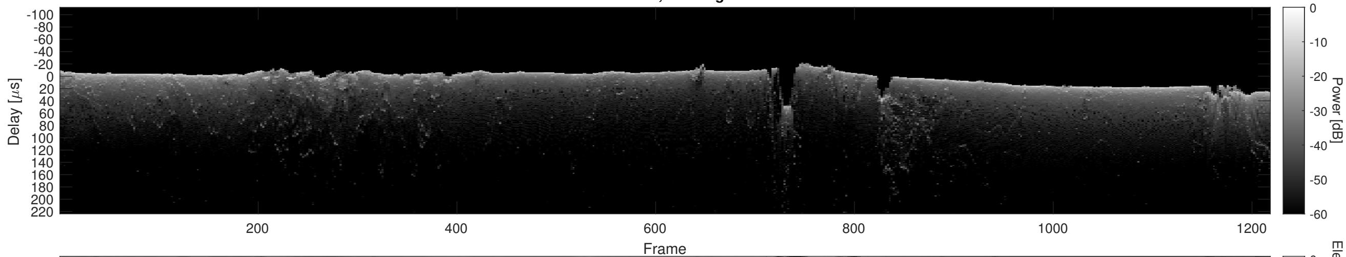
Orbit 23017, Cluttergram
