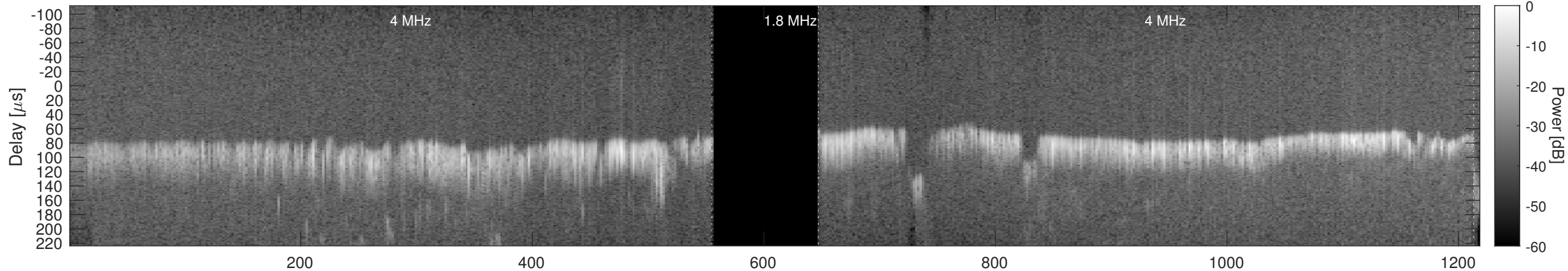
Orbit 23017, Window, Channel 2, Chapman
