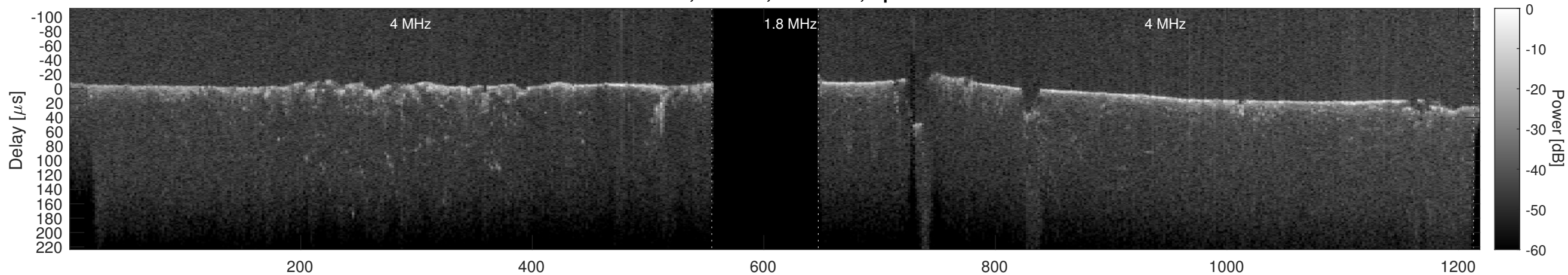
Orbit 23017, Cluttergram
