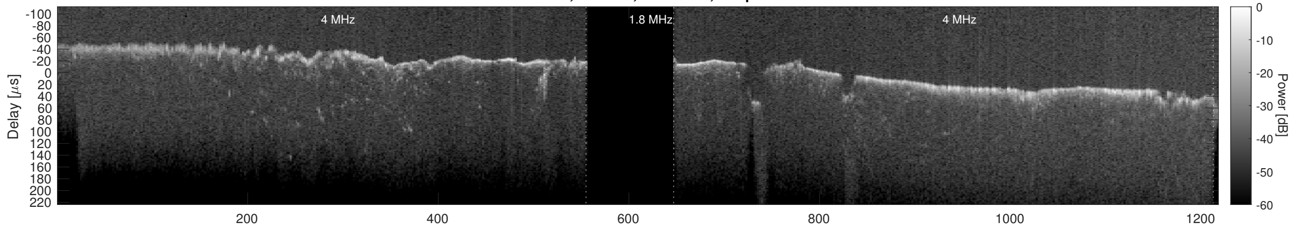
Orbit 23017, Window, Channel 2, Optimized
