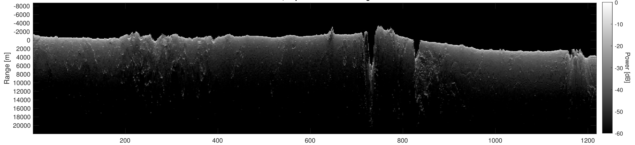
Orbit 23017, Depth-Corrected Cluttergram
