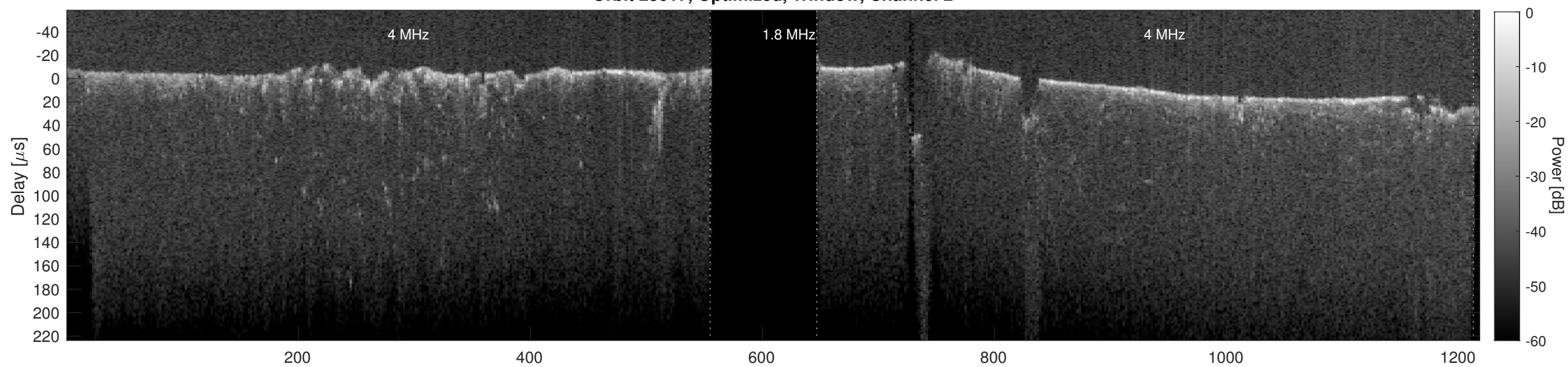
Orbit 23017, Cluttergram
