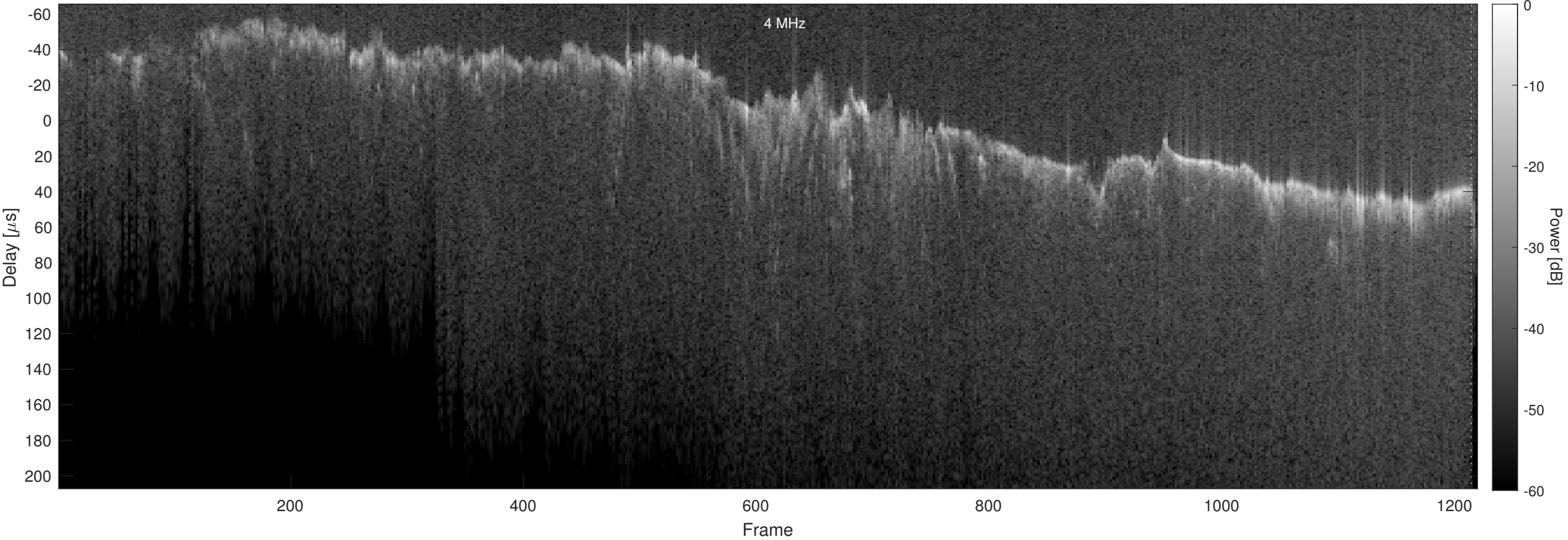
Orbit 23018, Chapman, No Window, Channel 2
