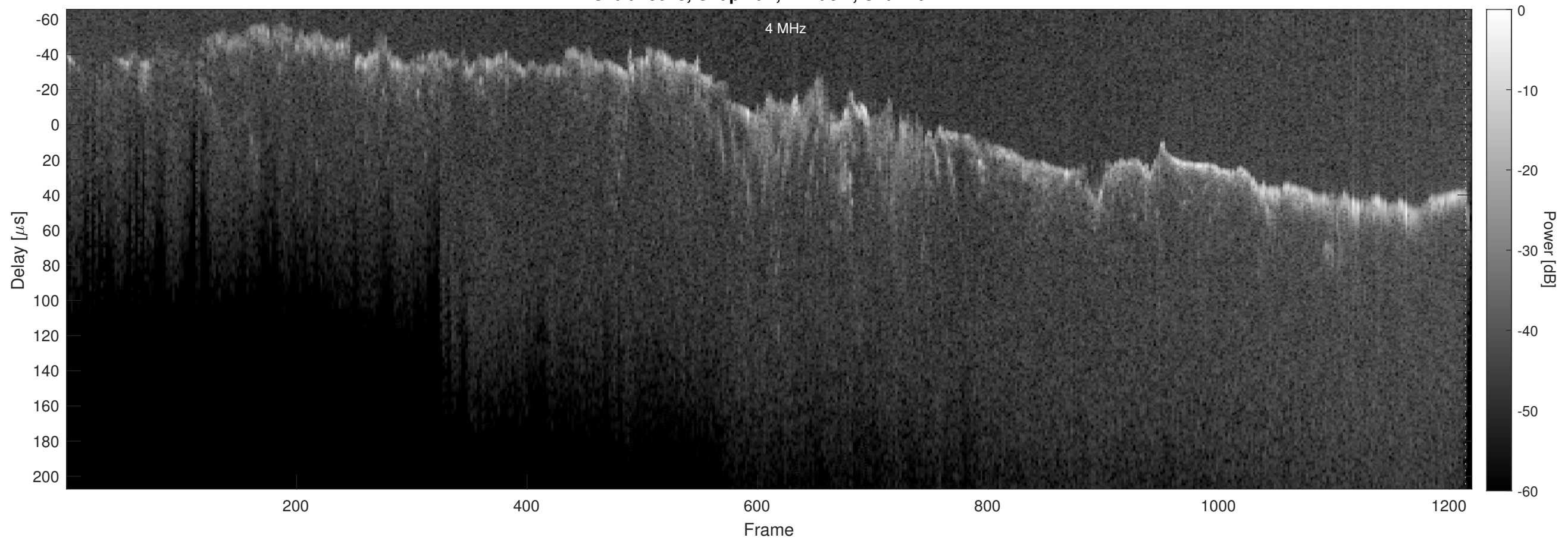
Orbit 23018, Chapman, Window, Channel 2
