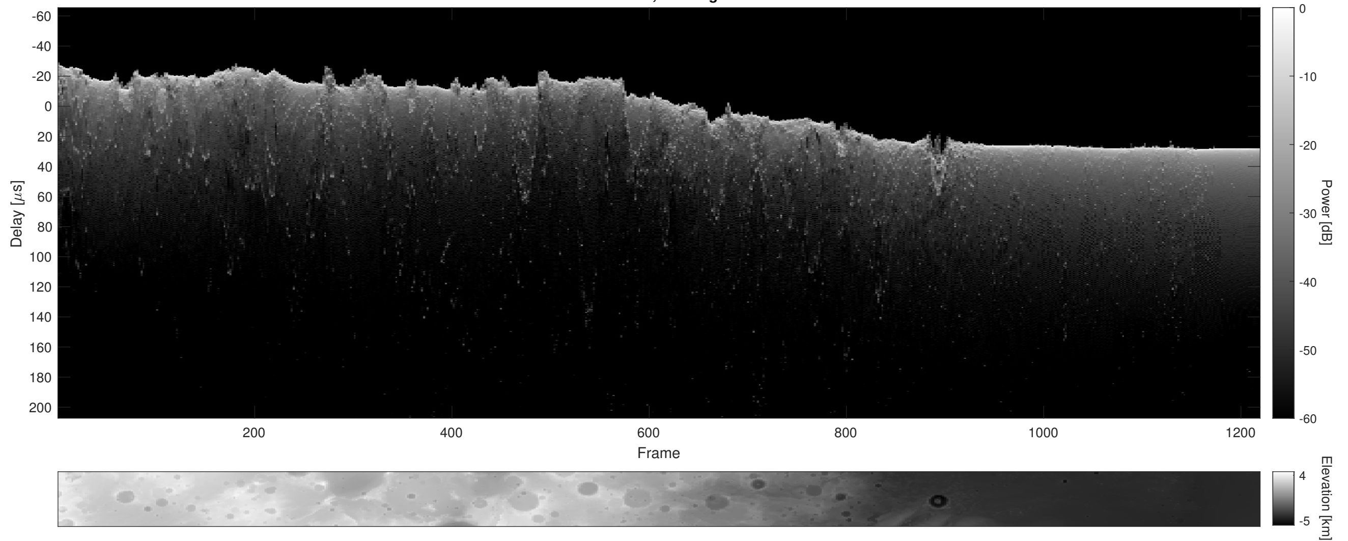
Orbit 23018, Cluttergram
