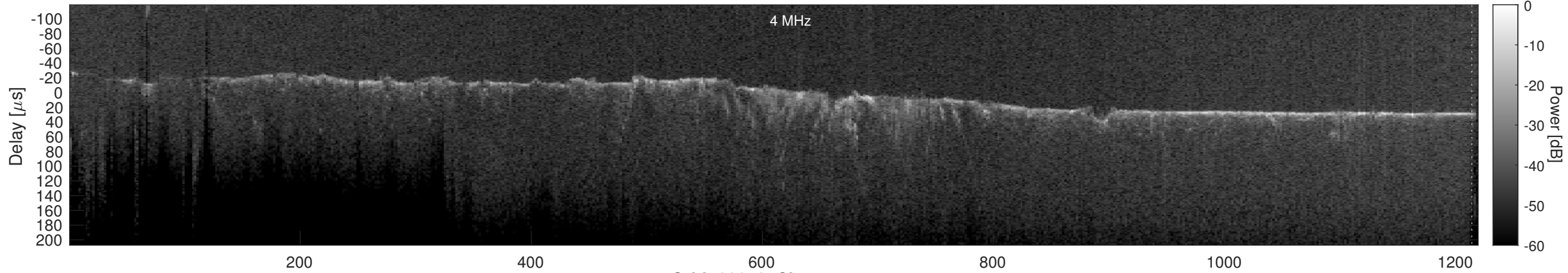
Orbit 23018, Cluttergram
