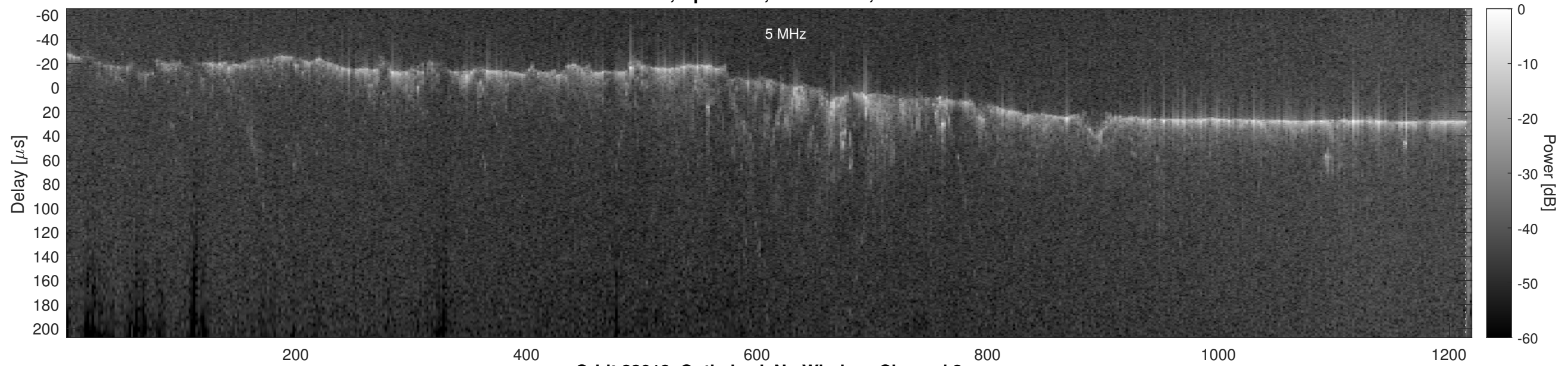
Orbit 23018, Optimized, No Window, Channel 2
