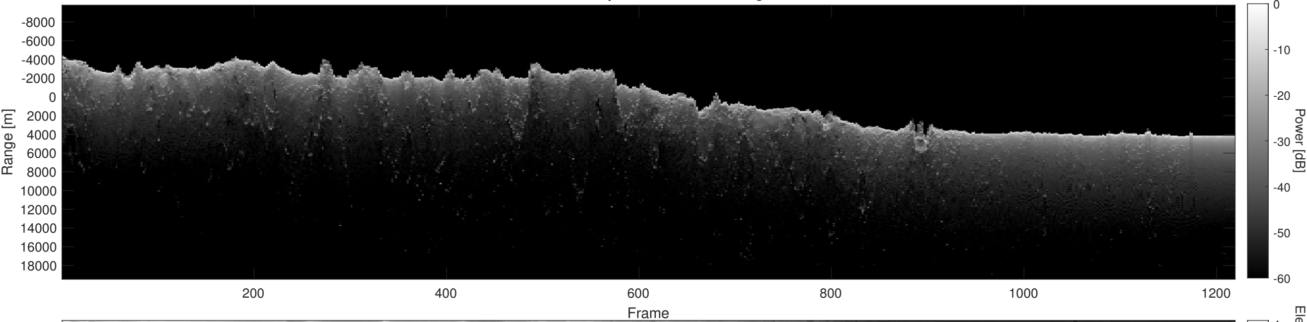
Orbit 23018, Depth-Corrected Cluttergram
