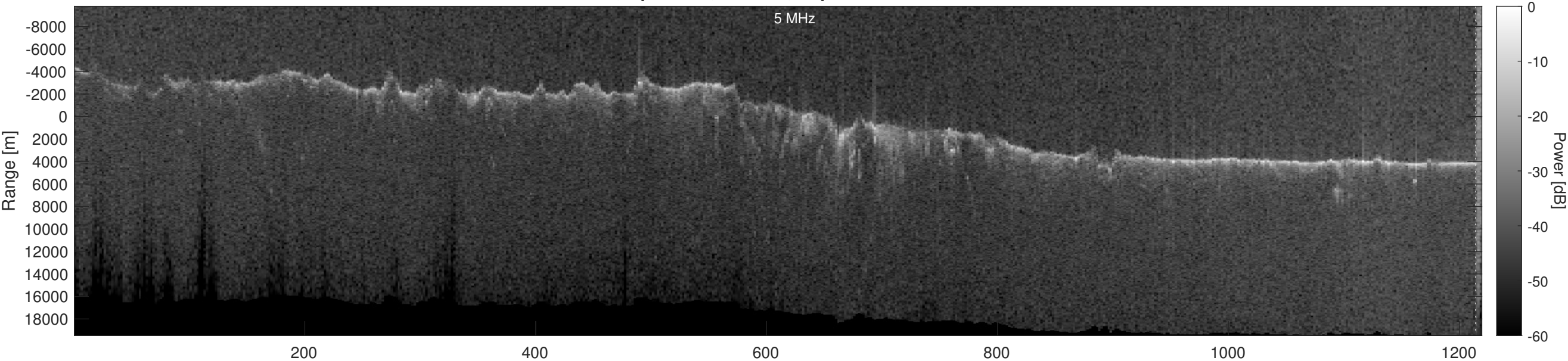
Orbit 23018, Optimized, Window, Depth-Corrected, Channel 2
