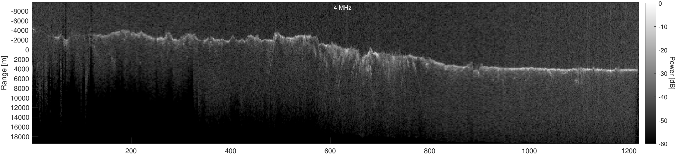
Orbit 23018, Depth-Corrected Cluttergram
