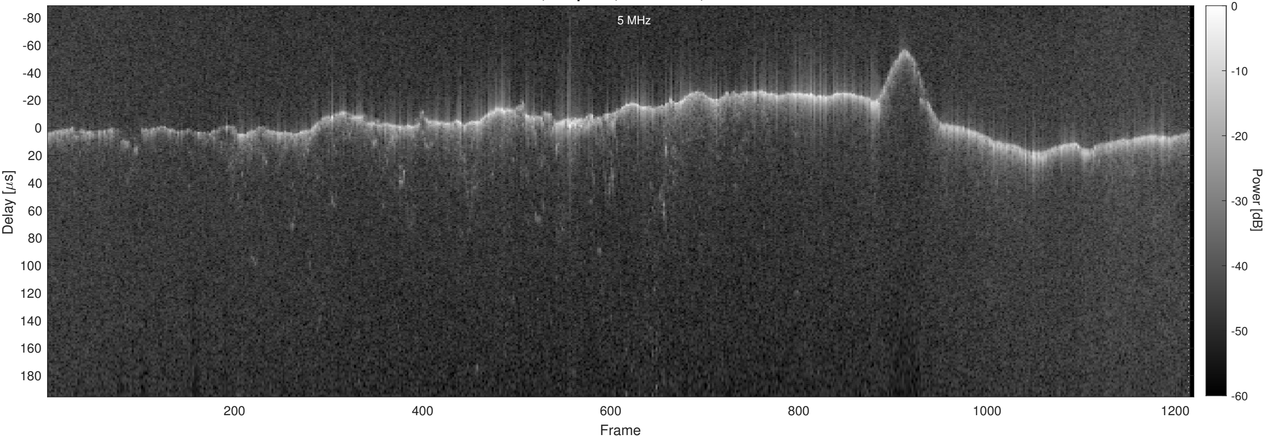
Orbit 23021, Chapman, No Window, Channel 2
