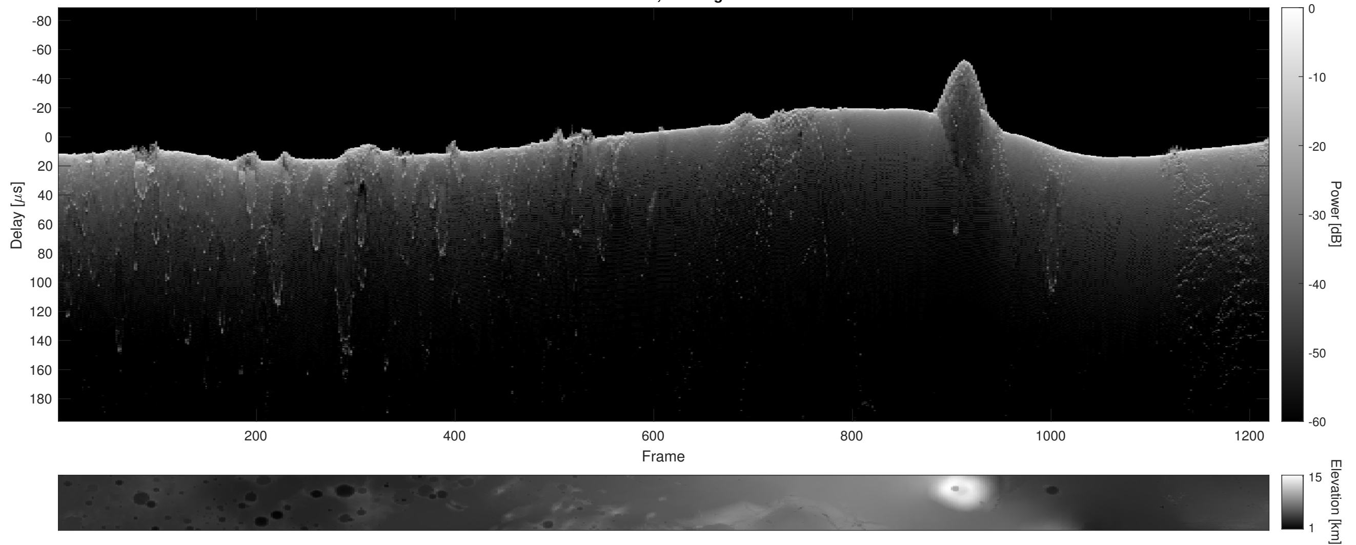
Orbit 23021, Cluttergram
